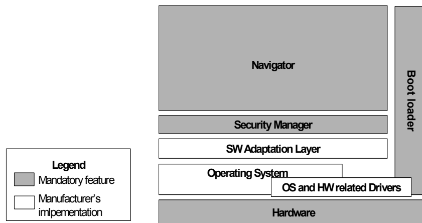
Figure 2.3: Possible software structure of a NorDig Basic IRD.
