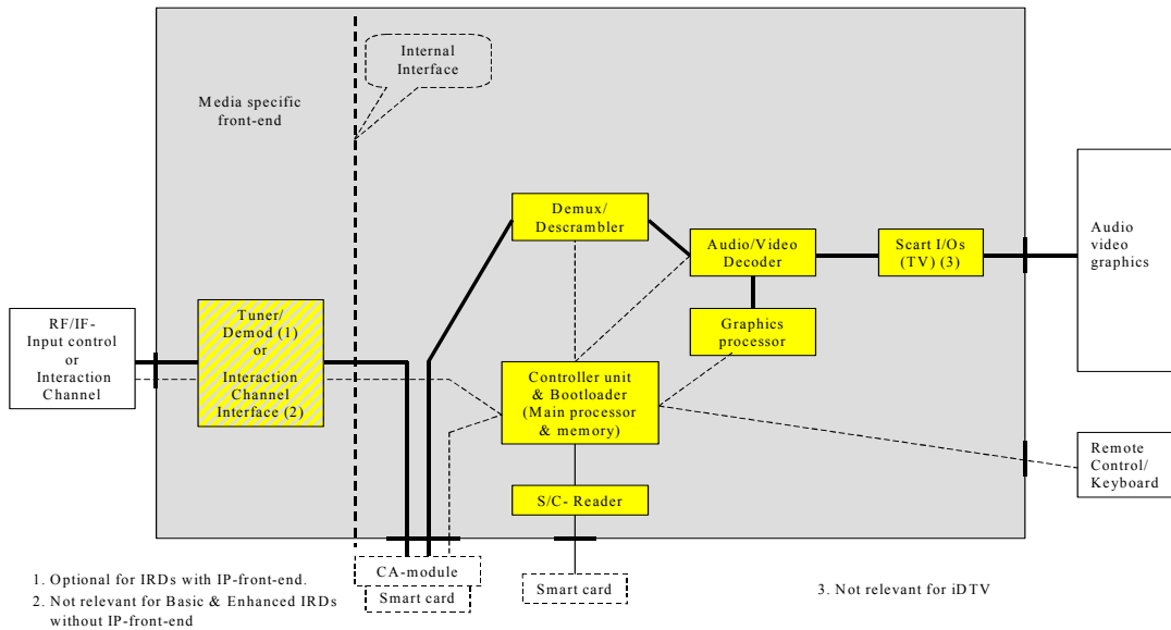
Figure 2.2 Functionality of Hardware and Firmware for NorDig Basic IRD
